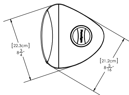
SPEAKER WITHOUT MOUNTING BRACKET
